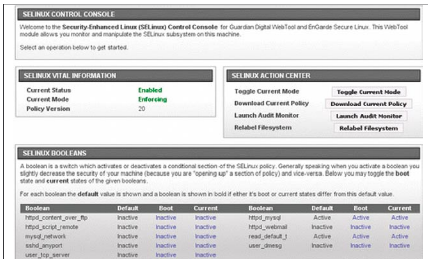
Figure 4. Selinux control
